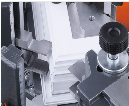
Hoekverbindingpers EP 124
