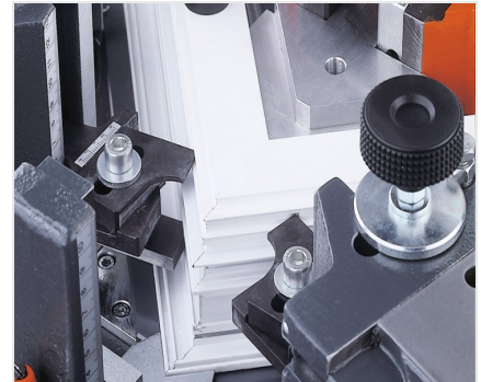
Hoekverbindingpers EP 124
