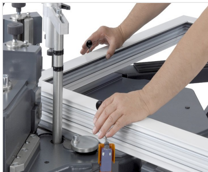
Hoekverbindingpers EP 124/20
