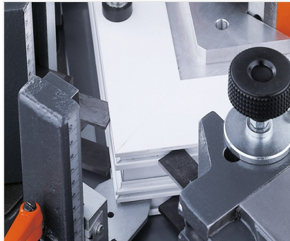
Hoekverbindingpers EP 124
