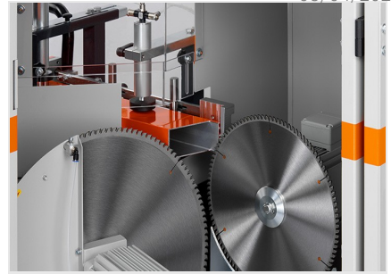
端面角切割机, AKS V-550
