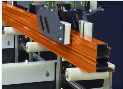
Cut-to-length centre SBZ 616/02
