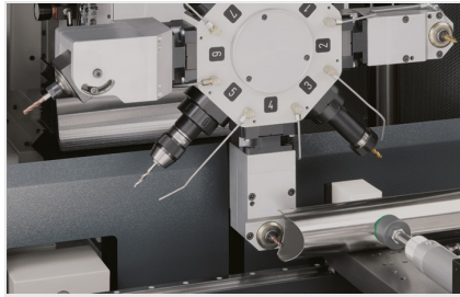
Profile machining centre SBZ 131 eluCam
