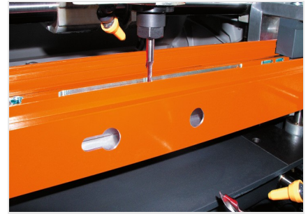
2-spindle copy router KF 78/23
