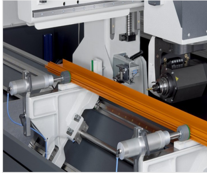
Profile machining centre SBZ 122/74
