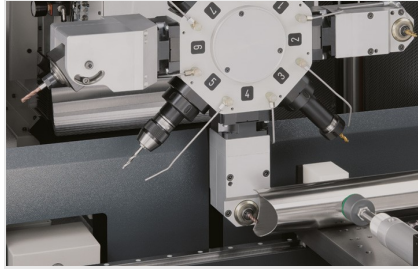
Profile machining centre SBZ 131 eluCam
