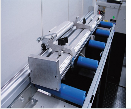
Length stop and measuring system AMS 200
